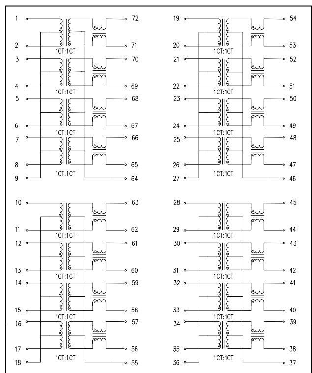
Schematic:HST-72002DR
